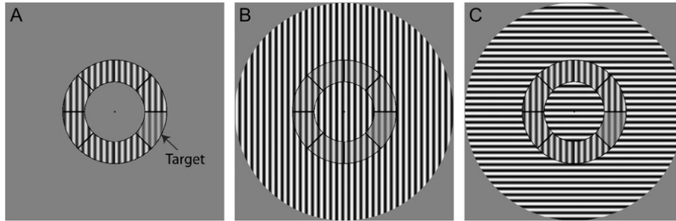
Fig. 1. Paradigm. Subjects performed a contrast decrement detection task in which they indicated whether they perceived a difference in contrast between any one segment (target) and the remaining 7 segments (pedestal) of the annulus. For half of the trials, the target had a lower contrast than the pedestal, which always had a constant contrast of 75%. In the remaining trials, all segments of the annulus displayed 75% contrast. The task was performed under 3 conditions: A) no surround, B) parallel surround, and C) orthogonal surround. The identical annulus is displayed in all 3 conditions in this figure.
