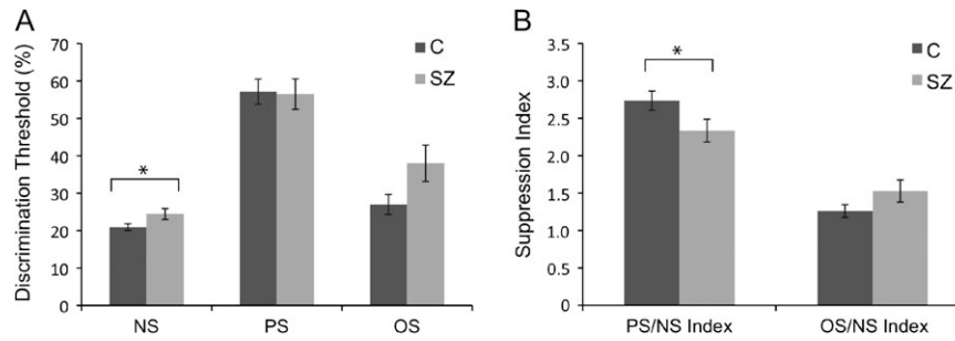
Fig. 2. Results. A) Contrast discrimination thresholds (the minimum contrast difference between target and pedestal segments necessary for accurate contrast discrimination) for no surround (NS), parallel surround (PS), and orthogonal surround (OS) conditions for patients and controls. *Significant group difference, P < .05 . B) PS/NS and OS/NS suppression indices for patients and controls. *Significant group difference, P < .05 .
